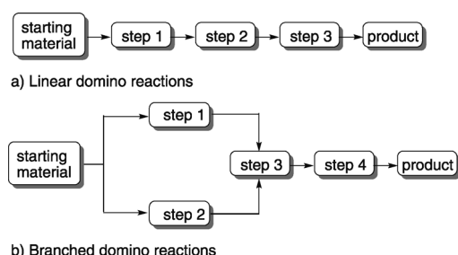
Figure 1. General sequences of linear and branched domino reactions.
