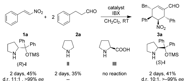
Scheme 3. Investigation of different amine catalysts.
