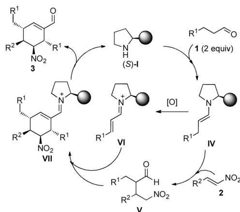
Scheme 7. Proposed catalytic cycle of the branched domino reaction through oxidative enamine catalysis.
