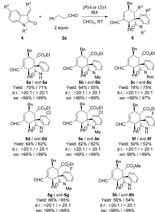
Scheme 6. The substrate scope of the reaction of aldehyde 2 with 2-(2-oxindolin-3-ylidene)acetate derivatives 4 to form the spiro compounds 5 .
