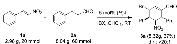
Scheme 5. The gram-scale reaction.
