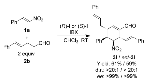
Scheme 4. The reaction of nitrostyrene with ( E )-5-phenylpent-4-enal.
